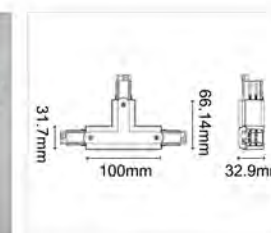
Right T joint
