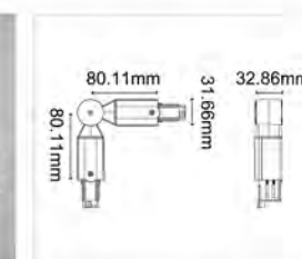
Outside L joint
