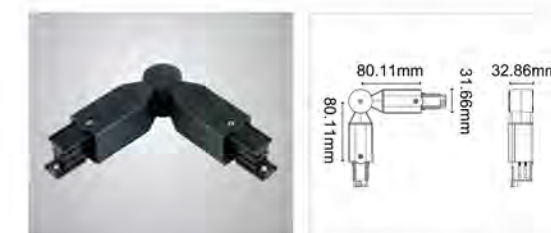
Inside L joint
